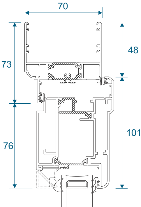
Open Out - AW607
