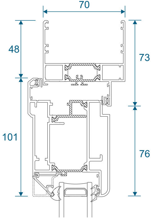
Open In - AW623
