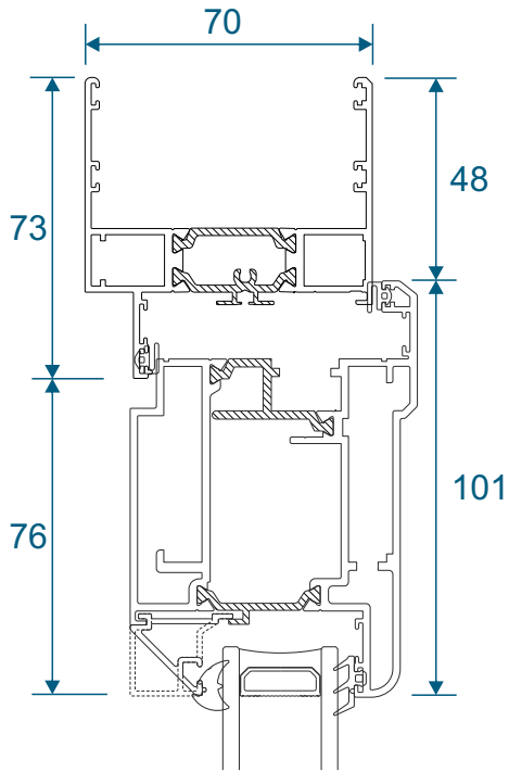
Open Out - AW623
