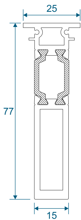
AW702 - 15mm Coupler For 70mm Frame
