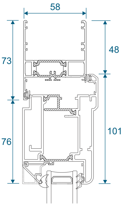
Open Out - AW608
