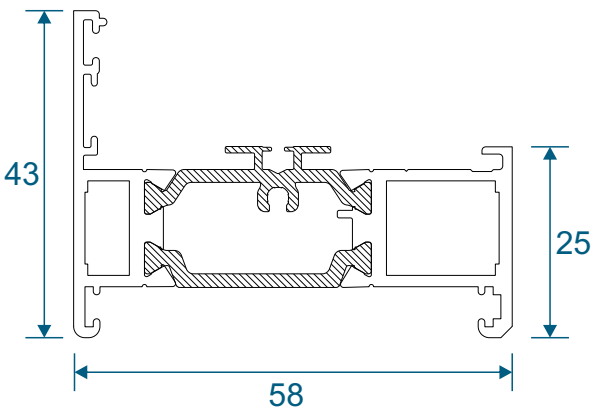
AW604 - Slim Equal Leg
