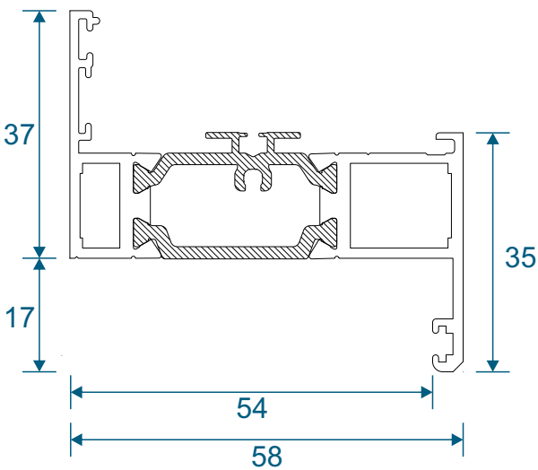
AW603 - Odd Leg (open out doors only)
