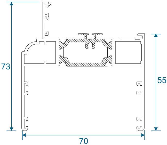
AW623 - Deep Direct Fix
