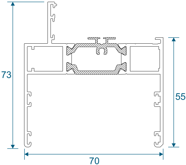
AW623 - Deep Direct Fix
