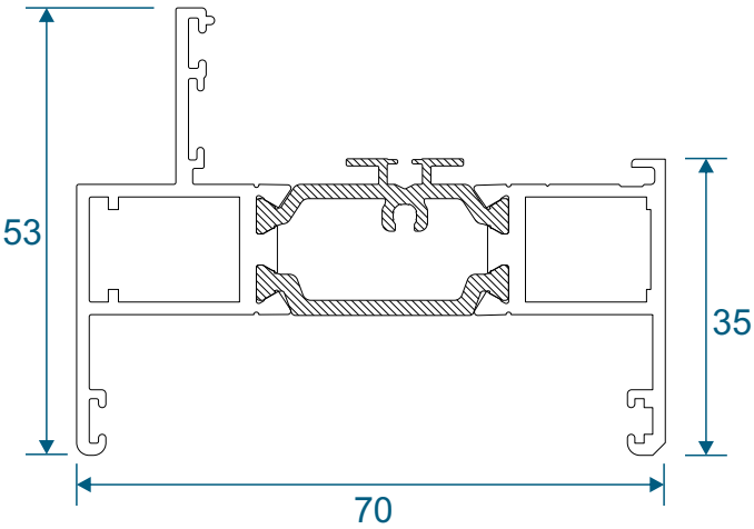
AW622 - Standard Direct Fix
